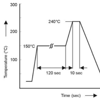
soldering condition
