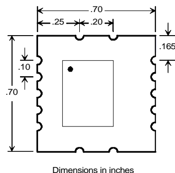
DR4000 Outline Drawing
